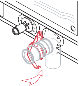
2 Fix the trap to the basin waste and secure the waste into rubber cone on the clamp waste fitting using silicone grease.
