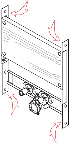
1 Refer to the fixing heights recommended for the basin and trap and use this information to mount the frame at the preferred height using the fixings provided.
