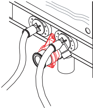
3 Connect the hot and cold water supply to the 1/2" brass angled back plate connectors as shown.
