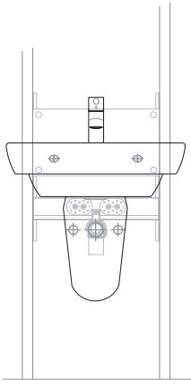
This In-Wall basin frame is designed to be mounted between vertical studwork i.e. it has no legs.
